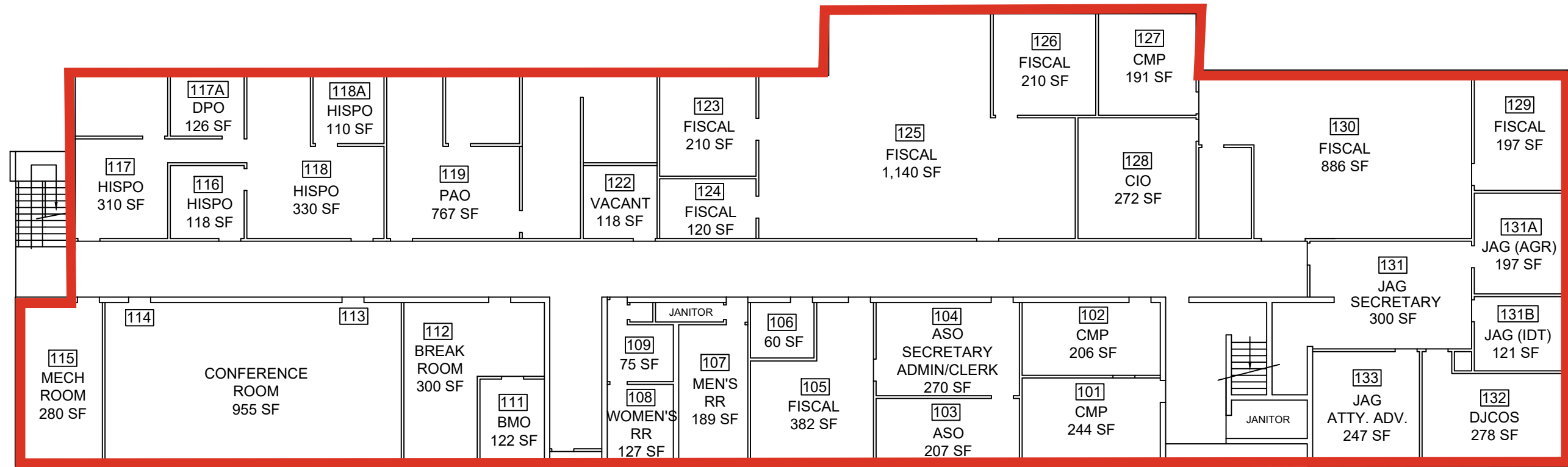
BUILDING 306 LOWER LEVEL PLAN
